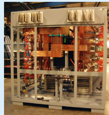
12 V 50 000 A thyristor controlled, water cooled
